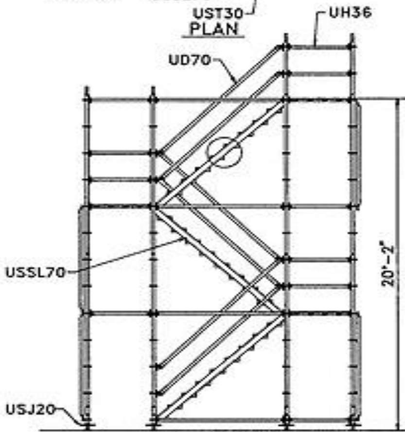
SIDE ELEVATION
