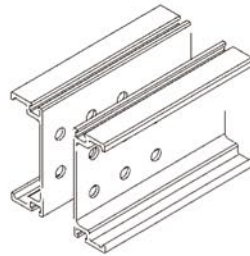
2 Aluma 55K Strongback ITEM NO. LENGTH FT. IN (MM) 122 Strongback Channel 8'6" (2591mm) 123 Strongback Channel 12'6" (3810mm) 124 Strongback Channel 16'0" (4877mm)
