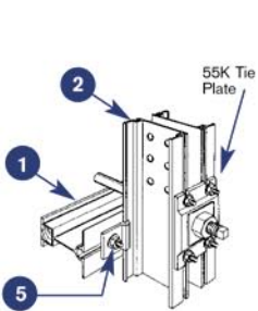
Beam/Strongback Connection
