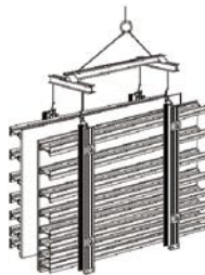
Typical Wall Form Section
